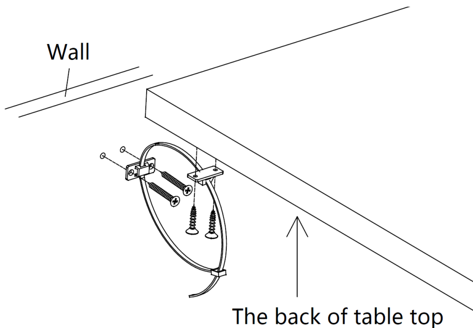
Mounting Plate x 2
